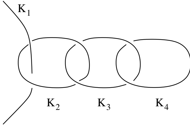
FIGURE 4. Handle decomposition for Proposition 7.2. Consider the link pictured above, where here K_1 is thought of as any initial framed knot in the three-manifold Y_1 , and K_2, K_3 , and K_4 are unknots with the property that K_i links K_{i-1} and K_{i+1} geometrically once (for i = 2, 3 ). The three cobordisms A_1: Y_1 \rightarrow Y_2 , A_2: Y_2 \rightarrow Y_3 , and A_3: Y_3 \rightarrow Y_1 which induce maps fitting into the long exact sequence are given as follows. A_1 is specified by the framed knot K_1 , A_2 is specified by the framed knot K_2 (thought of as a knot in Y_2 ) with framing -1 , while A_3 is specified by the framed knot K_3 with framing -1 . Three cobordisms B_2: Y_2 \rightarrow Y_1 , B_1: Y_1 \rightarrow Y_4 , B_4: Y_4 \rightarrow Y_2 are specified as follows. B_2 is specified by K_2 (thought of as a knot inside Y_2 ) with framing 0 , while B_1 is specified by K_3 with framing -1 , and B_4 is specified by K_4 with framing -1 . In particular, the cobordism B_2 \cup_{Y_2} A_1: Y_1 \rightarrow Y_1 is specified by the link K_1 \cup K_2 , where here K_2 is given framing 0 . In this composite cobordism, K_2 corresponds to a homologically non-trivial sphere with self-intersection number zero.
