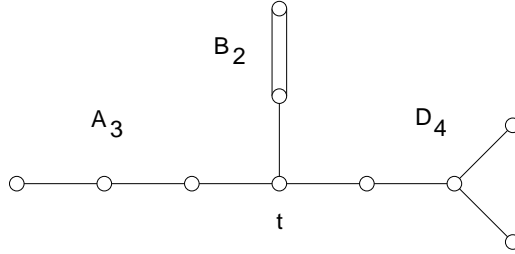
Figure 5. The join of A_3 , B_2 and D_4 .
