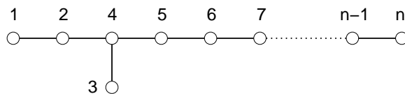
Figure 1. The E_n diagram.
